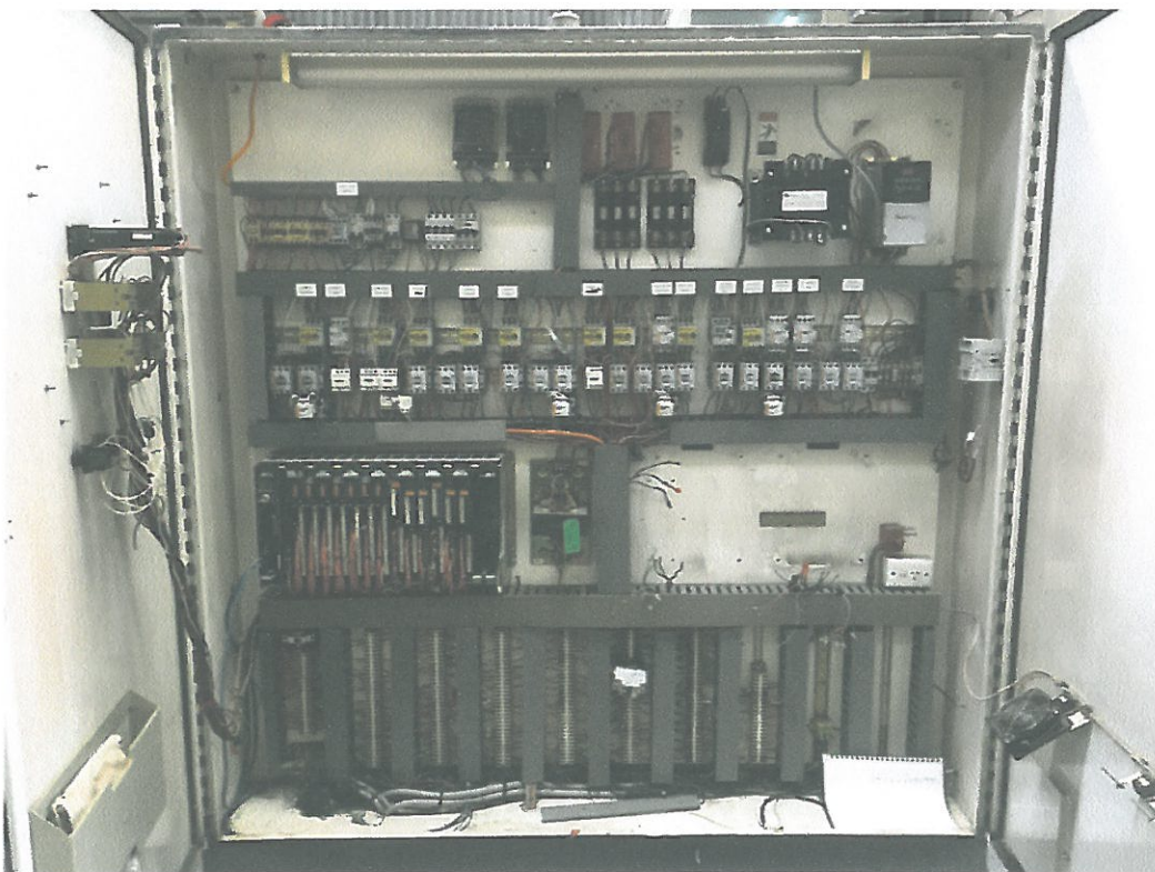
Bessermatic electrical panel
